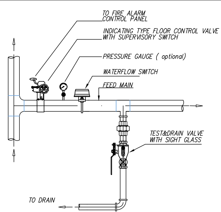
FLOOR CONTROL VALVE DETAIL
