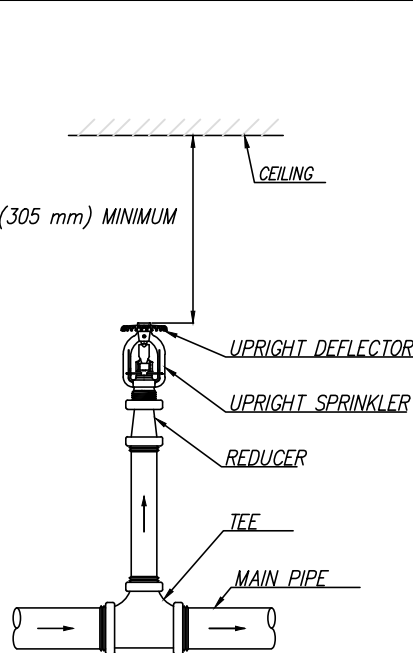
UPRIGHT SPRINKLER IN BUILDING SERVICE
