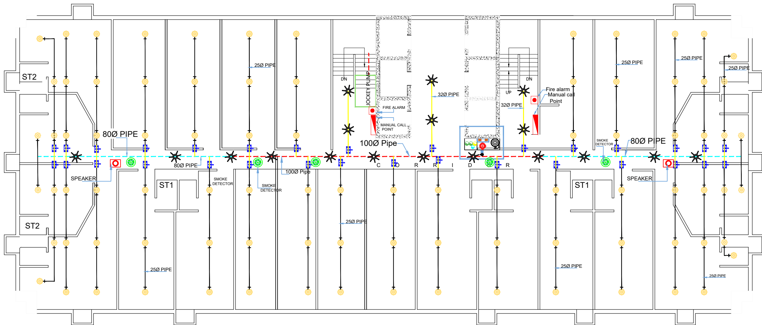
UPRIGHT SPRINKLER IN BUILDING SERVICE
